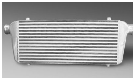
Intercooler Bar and Plate. core size 600L 300H 75W 3 inch inlet.
